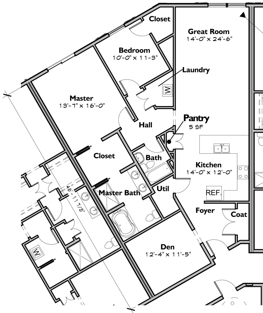
1 First Floor Unit Area Plan 3/32" = 1'-0"
